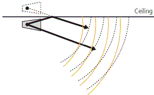
Figure 3: Acoustic mirroring of a conventional horn compared to the AXIS® ABF-260
