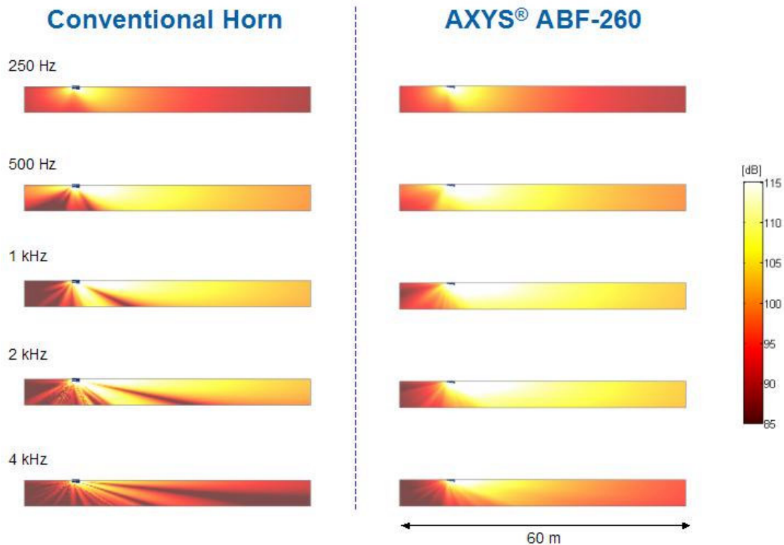
Figure 4: SPL distribution (direct sound+ceiling reflection) in the vertical plane in a tunnel for of a conventional horn mounted 0.2 m below the ceiling compared to the AXIS® ABF-260 (octave centre frequencies 250 Hz to 4 kHz)
