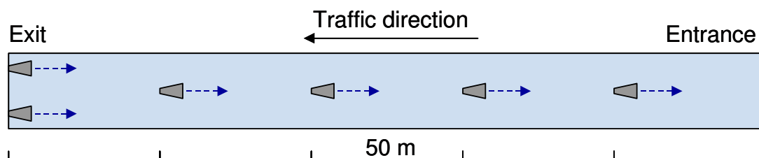
Figure 6: Typical ABF set-up for a "two-lane" tunnel tube (maximum width approx. 15 m).
