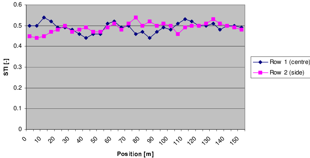
Figure 9: Measured STI values in the 15 m wide tunnel tube using optimised signal filtering and assuming 95 dBA fast traffic noise. Signal level is 103-105 dBA.
