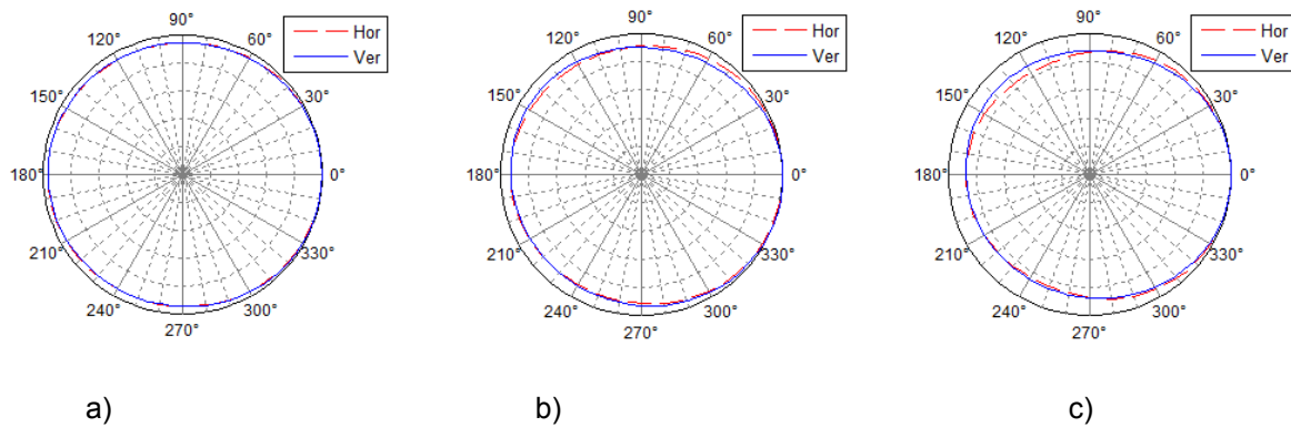
Figure 4: BEM-calculated polar diagrams @80Hz for a B-07 subwoofer facing different acoustic boundary conditions (scale: 6 dB/div): a) 'free-field' condition b) '3U1 full-space' condition c) '3U1 half-space' condition
