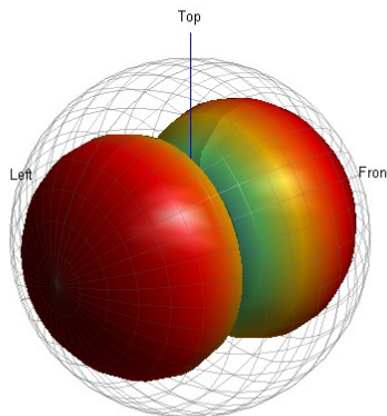
Figure 10: Desired dipole radiation pattern
