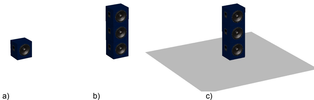
Figure 1: B-07 subwoofer facing different acoustic boundary conditions: a) As a single unit, 'free-field' condition b) First unit in a 3-unit array, '3U1' full-space condition c) As b) but ground-stacked, '3U1' half-space condition
