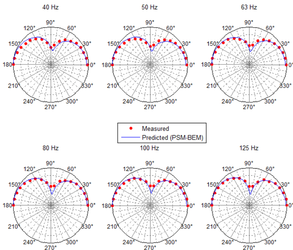
Figure 11: Measured and predicted horizontal polar data for a ground-stacked dipole subwoofer array of two cabinets.
