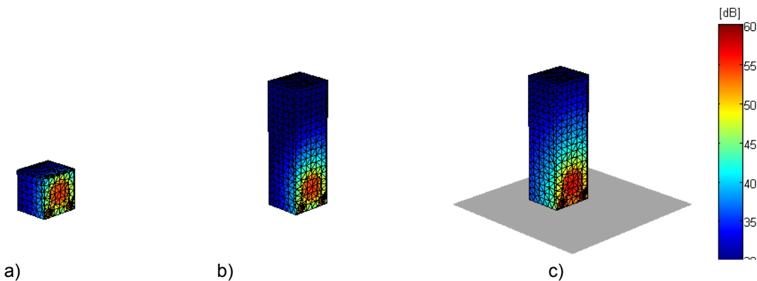
Figure 3: BEM-calculated SPL @80Hz for a B-07 subwoofer facing different acoustic boundary conditions: a) 'free-field' condition b) '3U1 full-space' condition c) '3U1 half-space' condition
