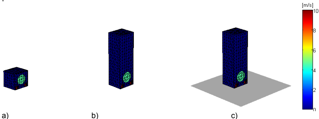
Figure 2: Measured normal particle velocity @80Hz for a B-07 subwoofer facing different acoustic boundary conditions: a) 'free-field' condition b) '3U1 full-space' condition c) '3U1 half-space' condition
