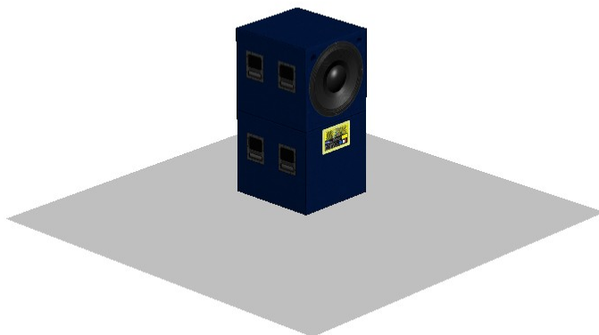
Figure 7: Differential subwoofer set-up of two B-121 units, placed on an acoustically hard ground plane
