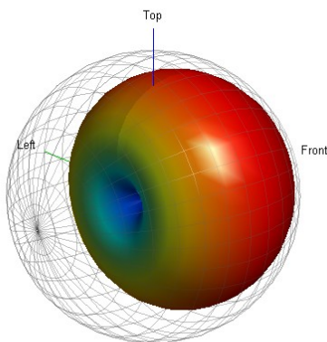
Figure 8: Desired cardioid radiation pattern
